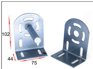
MANCAL TOLDO CORTINA CHAPA 2,5MM
