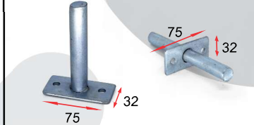
MANCAL PINO 5/8 CHAPA 2,5MM
