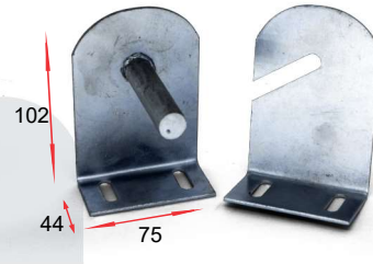
MANCAL TOLDO COM MOLA CHAPA 2,50 MM
